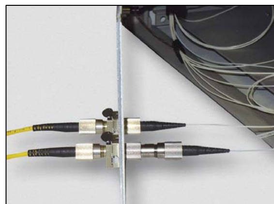
Fig. 4. MAS interface with OTA as sacrificial interface inside instrument.
