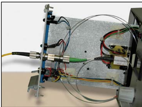
Fig. 1. UGT as sacrificial interface inside instrument.
