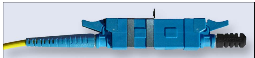
Fig. 6. Optical Reflection Module (ORM) (right).
